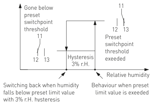
Switching output 1
