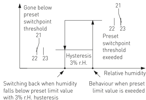
Switching output 2
